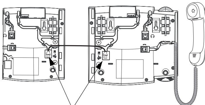
RJ-45 Connectors
