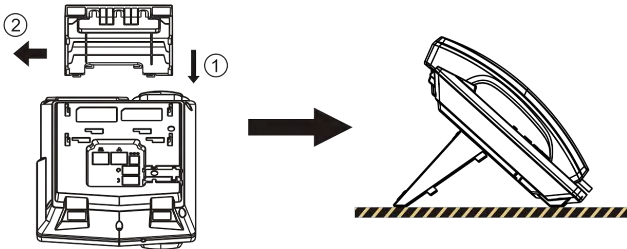
Figure 1 - Desktop Installation
