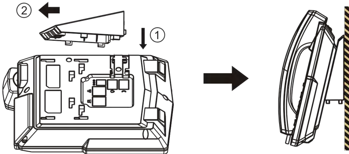
Figure 2 - Wall-mount Installation
