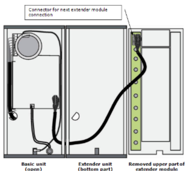
8-Button Extender Module Connection to Basic Unit
