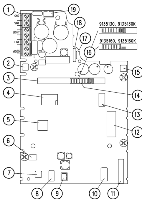
PCB Layout, Version 10
