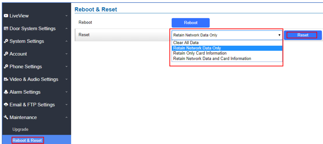
Figure 92: Reset via Web GUI
