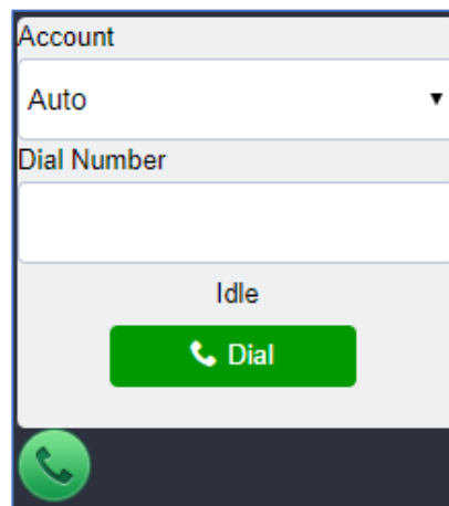
Figure 64 : Click-To-Dial
