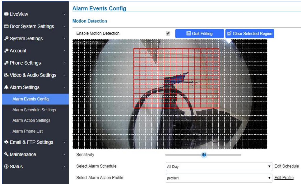
Figure 71: Region Config
