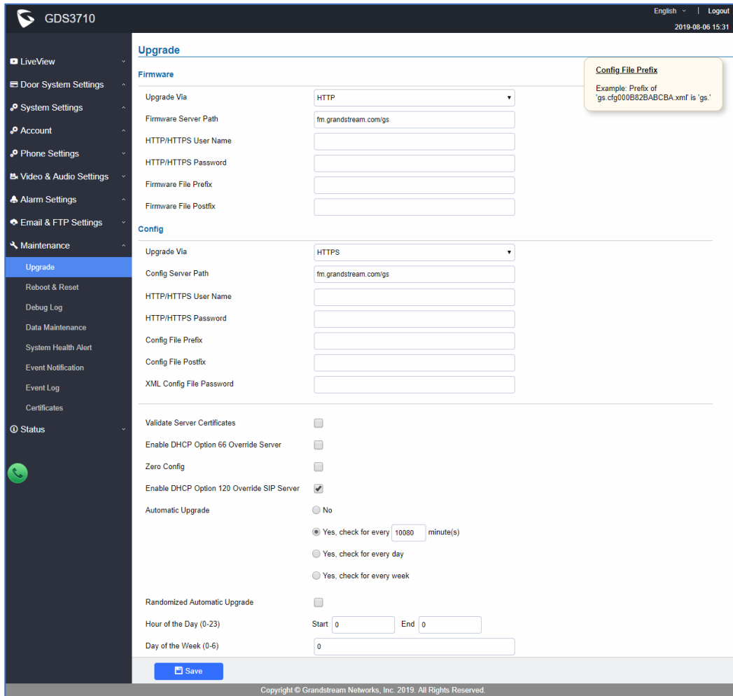
Figure 81: Upgrade Page
