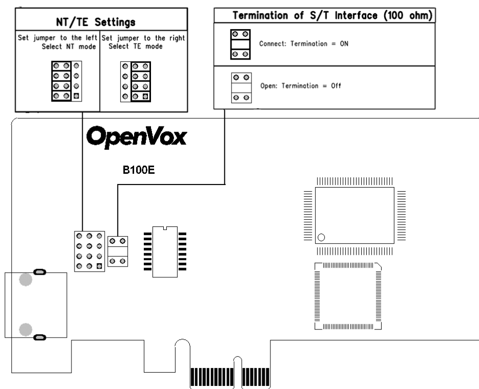
Figure 3 Jumper setting
