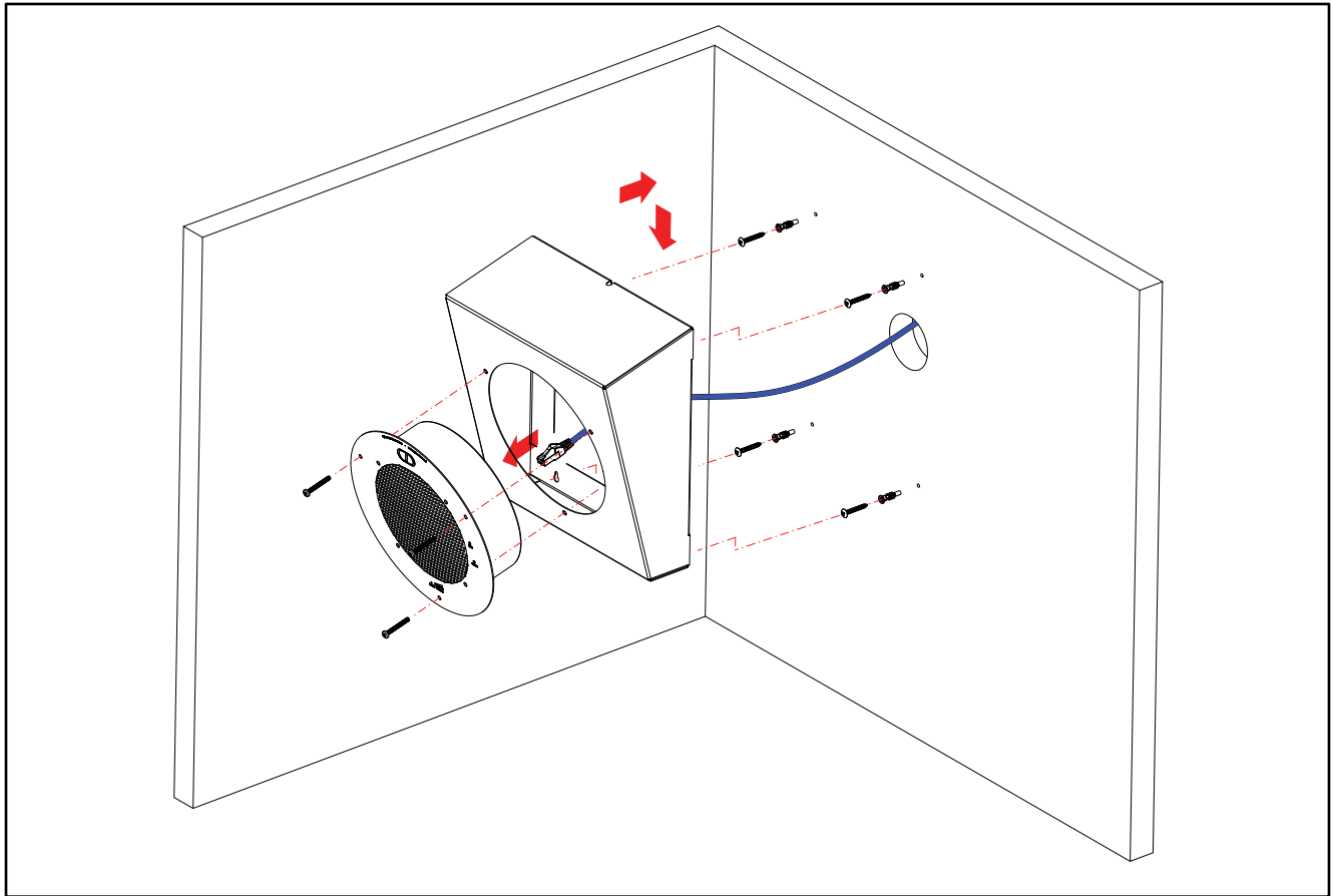
Exploded View
