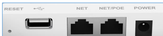
Figure 1: GWN7610 Ports
