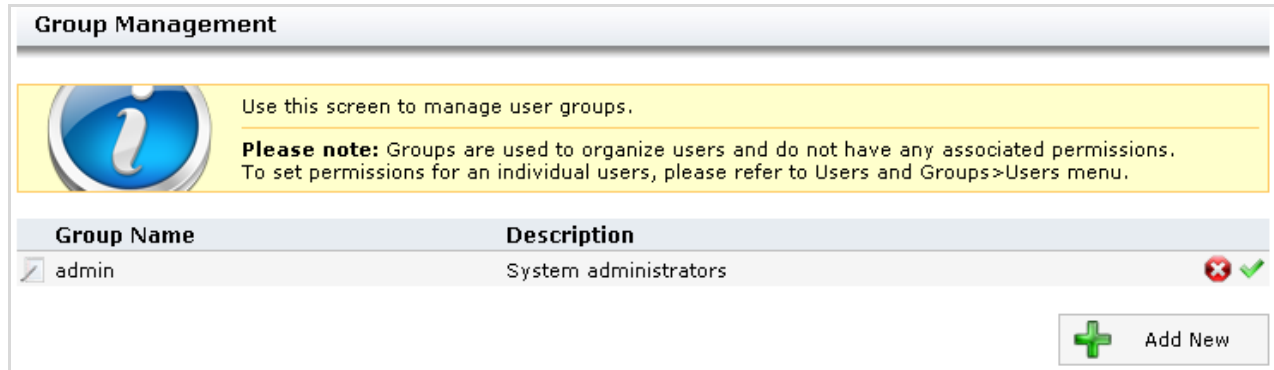
Image 73: Group management
