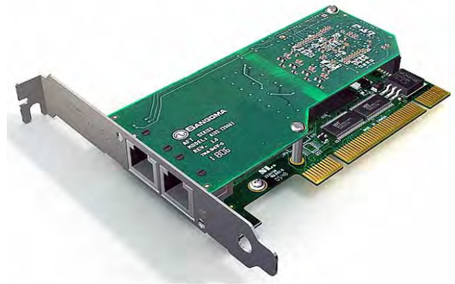
A102 2-port T1/E1/J1 board shown with available PCI Interface
