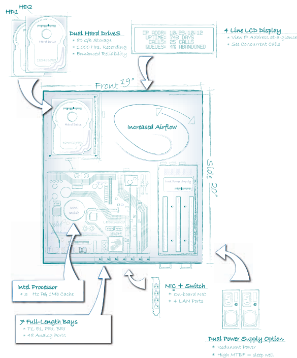
trixbox Appliance Top View
